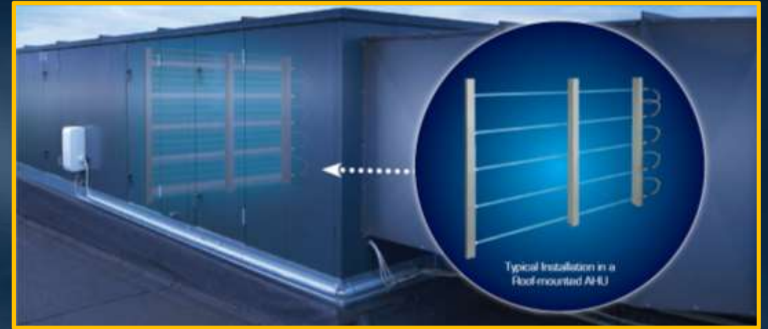
Typical UV light installation in air handling unit
